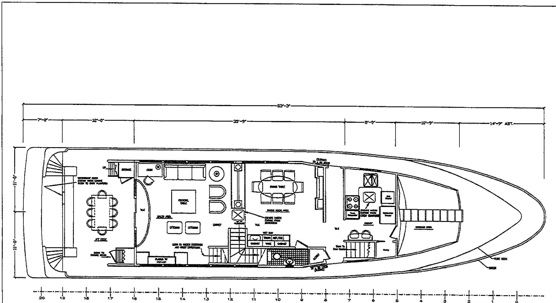
MAIN DECK PLAN VIEW
